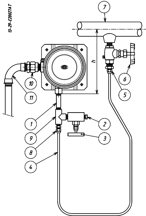
Fig. 9 - Example of mounting -
