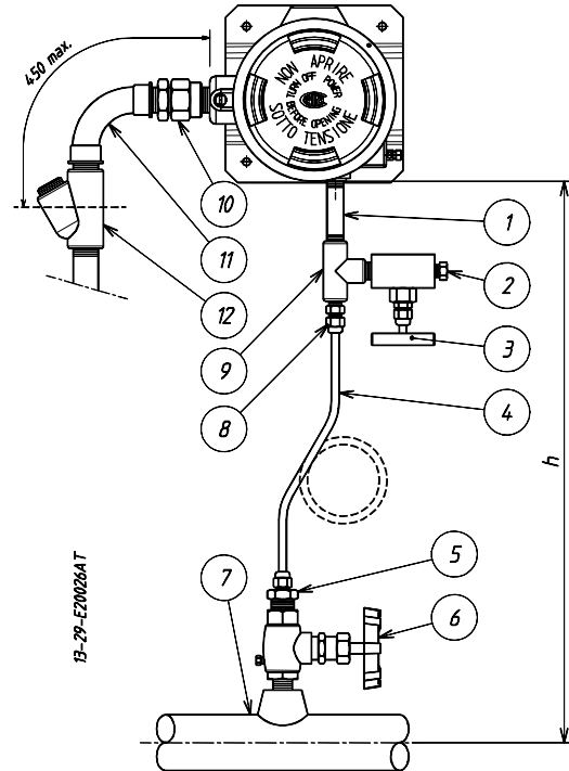
Fig. 8 - Example of connections -
