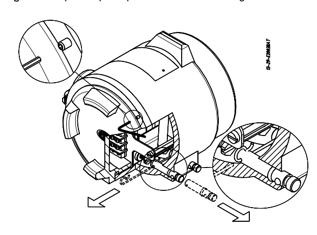
Fig. 4 - Explosionproof pressure switch blocking device
