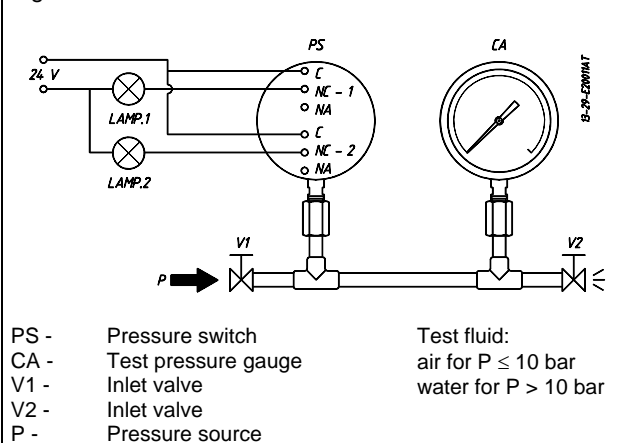
Fig. 5 - Calibration circuit
