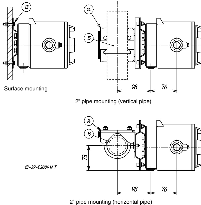
Fig. 9 - Example of mounting -
