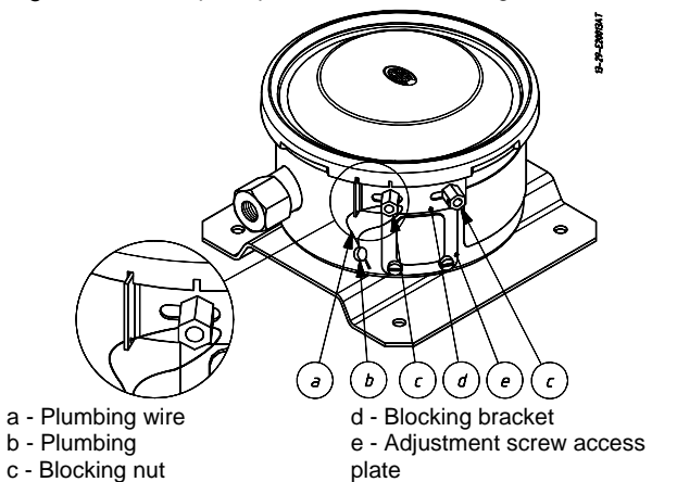
Fig. 3 - Weatherproof pressure switch blocking device -
