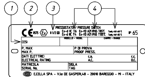
Fig. 1 - Explosionproof instruments plate
