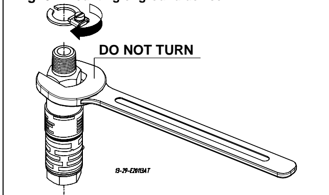
Fig. 6. Mounting of ground device
