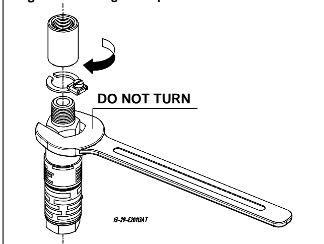
Fig. 7. Mounting of adaptors
