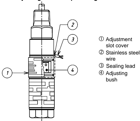
Fig. 2. Adjusting bush and plumbing
