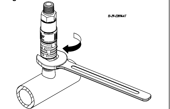
Fig. 5. Pressure connection
