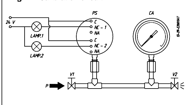
Fig. 4. Calibration circuit
